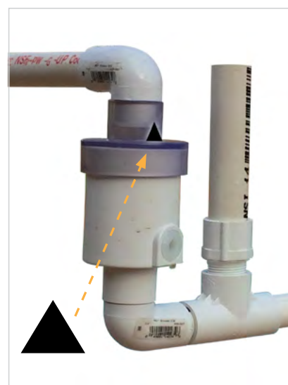
Figure 3 - N-Series Air-Trap positive pressure orientation is vertical
