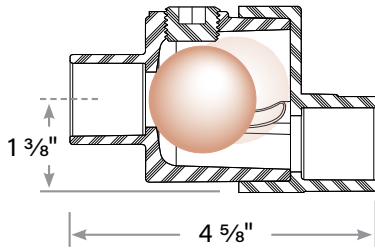
Positive Pressure Orientation
