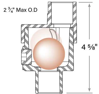
Positive pressure orientation
