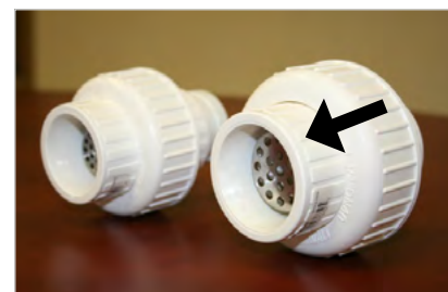
Figure 5 - In-line Union-Strainers. Install in the drain line upstream of the Air-Trap. This will aid in preventing debris from entering trap. The arrow shows the direction of water flow, into the strainer basket.
