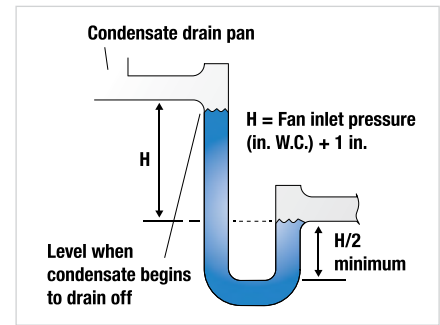
Figure 1c: Condensate Draining
