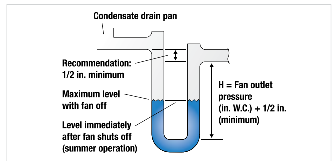
Figure 1e: Fan Off - High & Low Level
