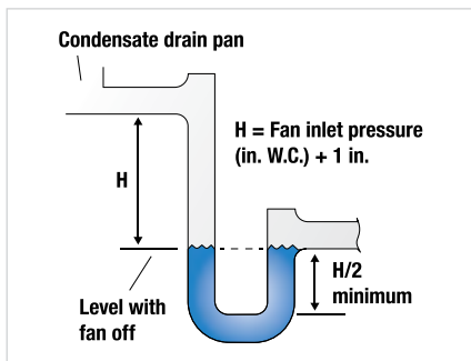
Figure 1a: Fan Off
