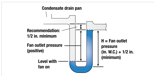
Figure 1d: Fan On - Condensate Beginning to Drain
