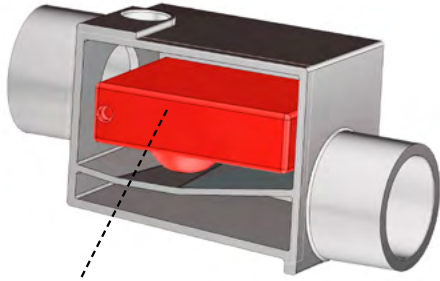
Levered, horizontal pancake designed float-valve with a mechanical advantage about a pivot point
