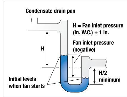
Figure 1b: Fan Just Started
