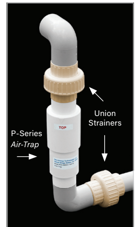
Union Strainers conjoined with a P-Series HVAC Air-Trap
