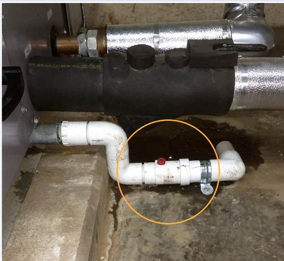
N-Series, commercial mechanical room negative pressure installation.
